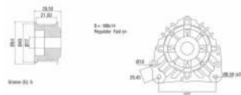
Pulley Terminal Connections Housing
