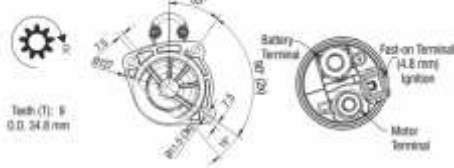
Starter Drive
