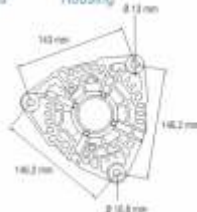
Housing
