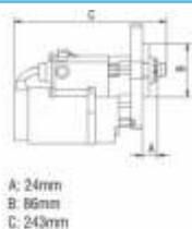
Starter Solenoid
