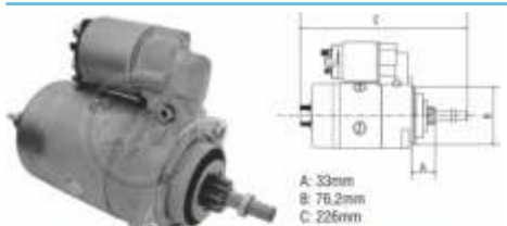
Starter Drive
