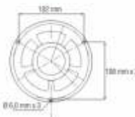
Housing
