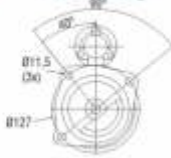
Drive Housing
