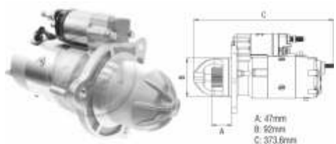
Starter Drive
