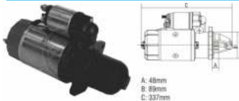
Starter Drive
