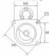
Drive Housing
