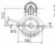
Drive Housing
