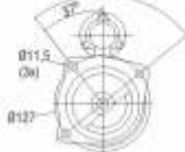
Drive Housing
