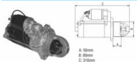
Starter Drive
